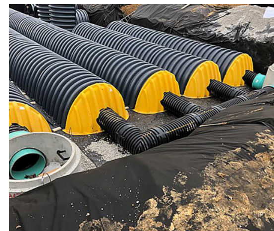
B : UNDERGROUND STORAGE Highly impervious light industrial and residential sites may use underground storage methods to effectively manage the sites' stormwater loads.
